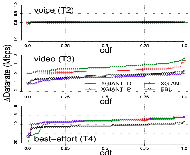
Fig. 12. Difference in mean datarate in 80-eNB scenario
