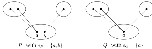
Fig. 17. Example of merging in an existential pattern P to produce the existential pattern Q .
