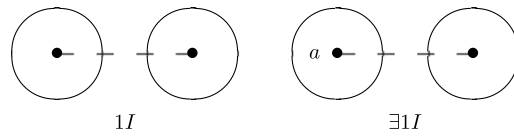
Fig. 14. A simple pattern 1I and an existential version \exists 1I of the same pattern.
