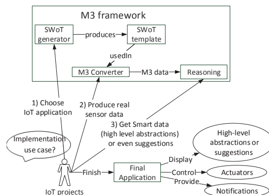
Figure 5: The SWoT generator of IoT applications
