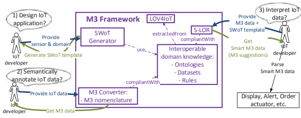
Figure 1: Assist developers in building IoT applications with M3 and the SWoT generator
